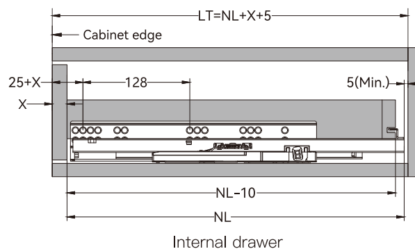
Drawer size and drilling(mm)
