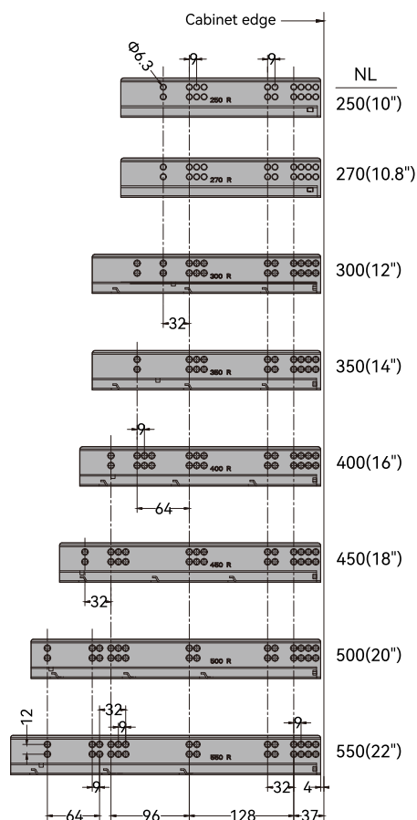
Hole positions(mm)
