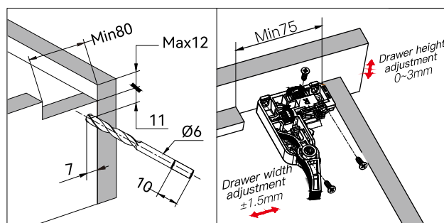
Installation steps for stablizer bar:
