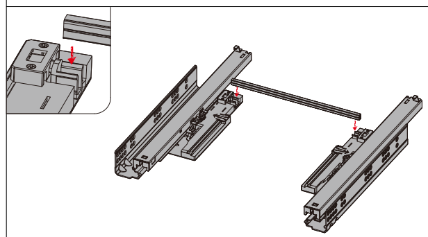
Installation steps for stablizer bar:
